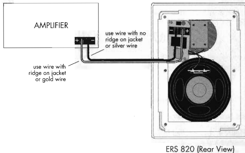
Figure 3. Example of correct wiring connections used on the Infinity ERS Model 820.
